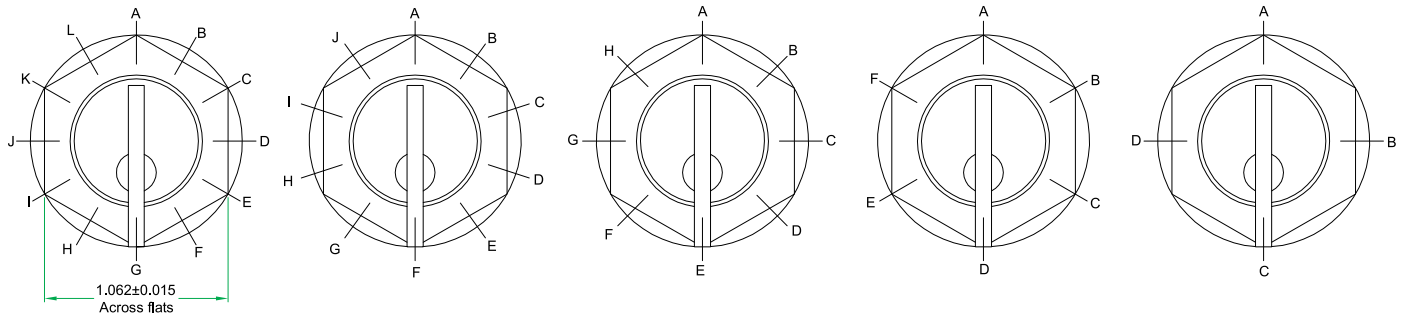
30° INDEXING
